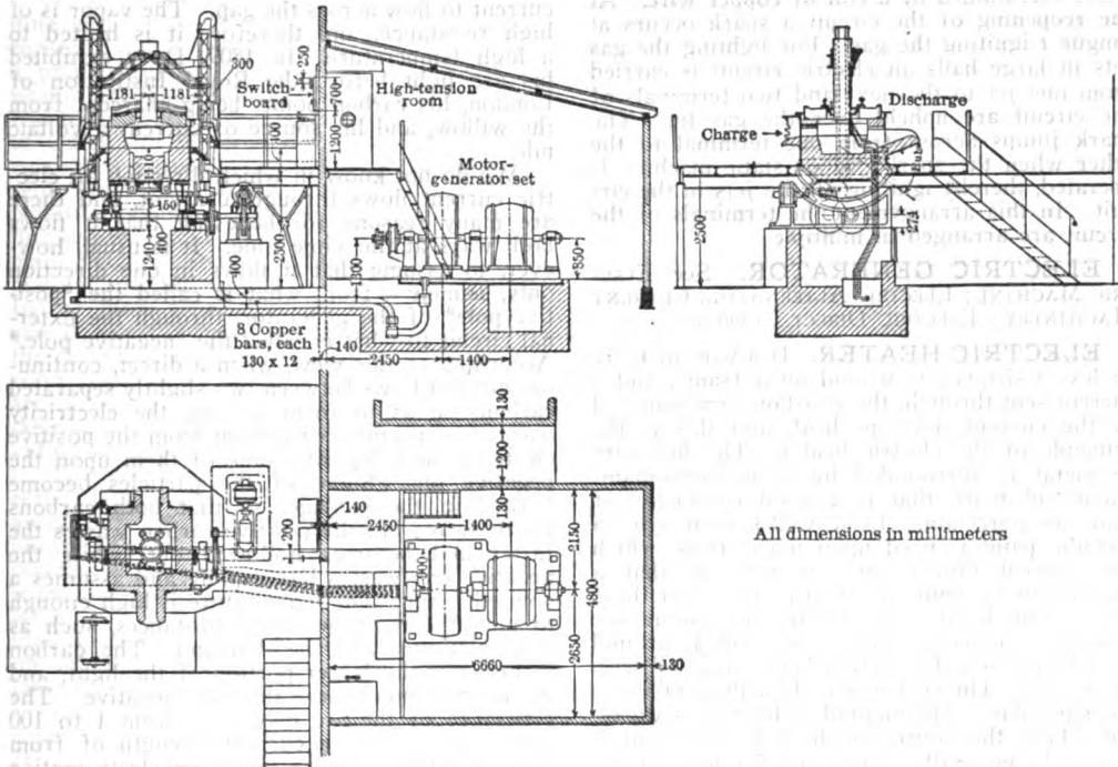
Arrangement of electric-furnace steel plant, Oberhausen, Germany.
