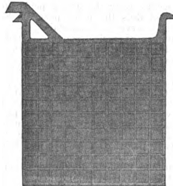
FIG. 9. Box Negative Plate—General Stationary Service—1-10 size.
