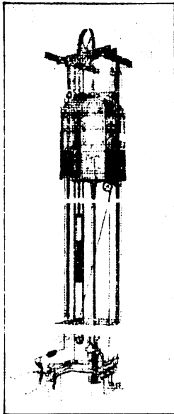
FIG. 3.—Plunger passenger elevator lever control.
