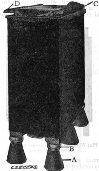
FIG. 28. Large Stationary Cell. Stand-by Service. Contains 45 plates as in Fig. 29. Approx. 1/20 size.
