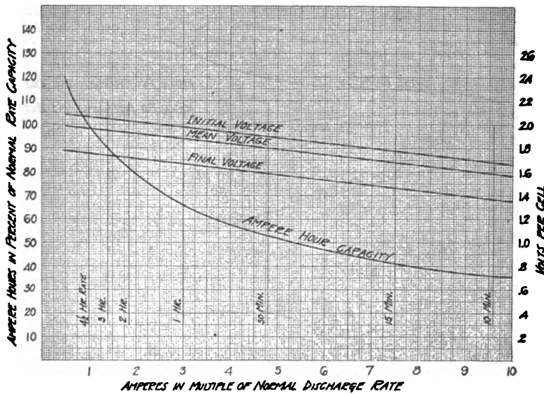
VOLTAGE vs CAPACITY CHARACTERISTICS OF LEAD CELL
