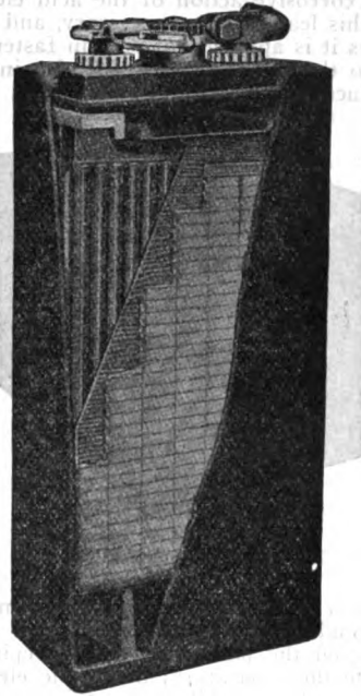
FIG. 24. Ironclad Exide Cell for Vehicle and General Service. About 1/5 size.
