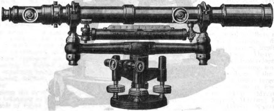
Engineer's Wye Level.
