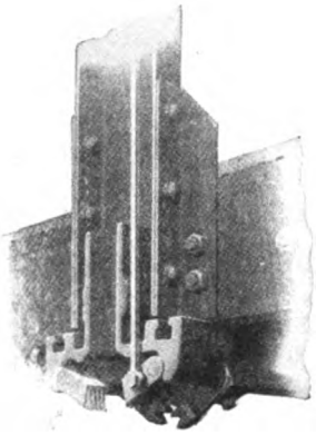
9 Detail of Safety for Wood Guides
