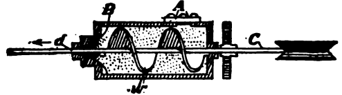
FIG. 1.—Rubber Covering Machine.
