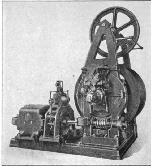
6 Direct Current Single Screw Electric Elevator Machine
