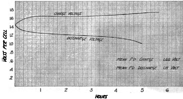
TYPICAL CHARGE & DISCHARGE CURVES OF EDISON CELL-NORMAL RATE
