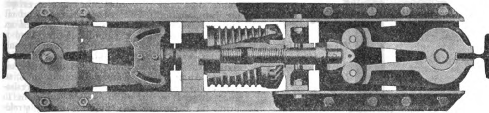
FIG. 13.—Wedge clamp safety.
