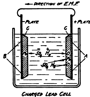
CHARGED LEAD CELL
