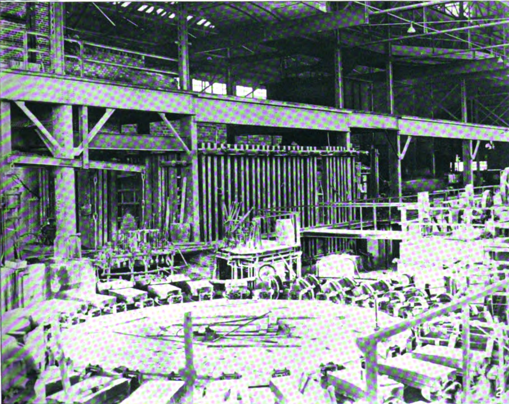
1 Electrolytic process of copper-refining, showing tanks filled with a solution of copper sulphate and containing sheets of copper connected to the terminals of a generator 2 Casting side of a furnace showing copper anodes placed radially on a Clark casting machine
